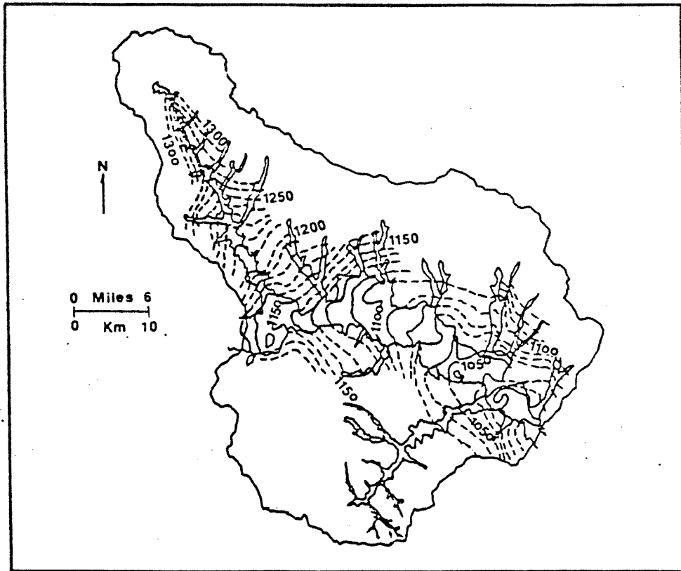
Figure 16. Water Table Map, Modeled Reach 3. (after Silka, 1975)
