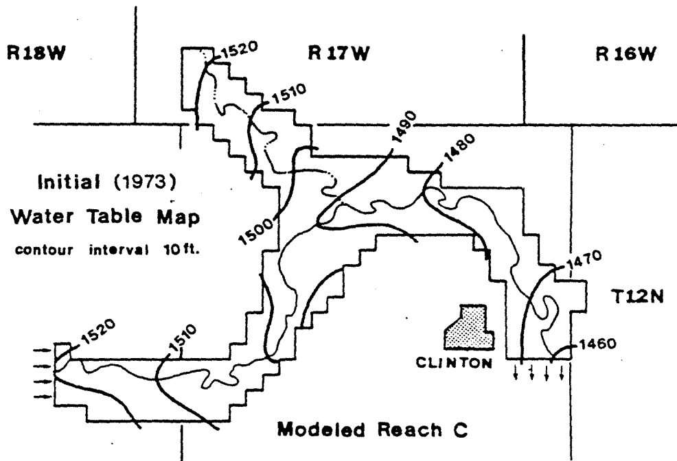
Water Table Map, July 1, 1973, Subreaches B and C, Modeled Reach 1.
