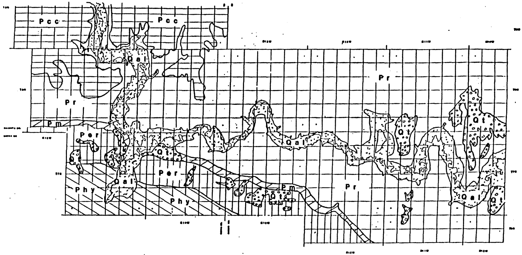
Figure 8. Geologic Map Reach 2 Subreach B
