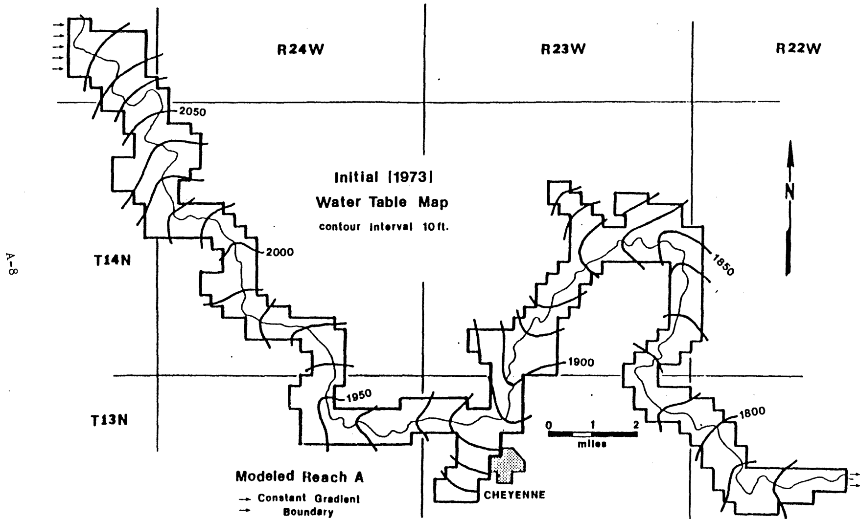
Water Table Map, July 1, 1973, Subreach A, Modeled Reach 1.
