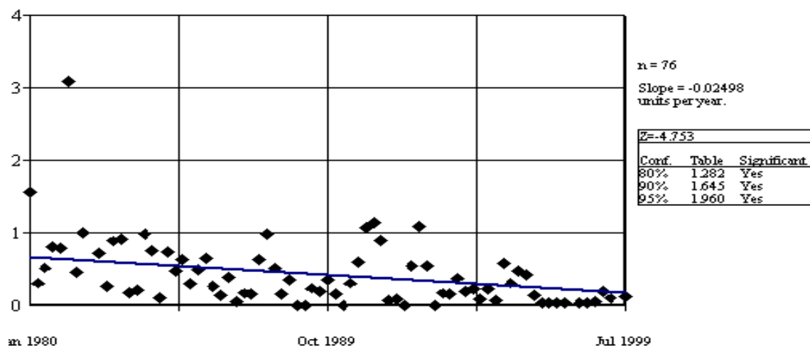
Figure 22. Trend analysis for total phosphorus data collected from January of 1980 through July of 1999 at the North Canadian River near Yukon. Slope calculated using the Seasonal Kendall slope estimator. Data deseasonalized based on four seasons beginning January 1, April 1, July 1, and October 1. Values on Y-axis are LOWESS calculated residuals.
