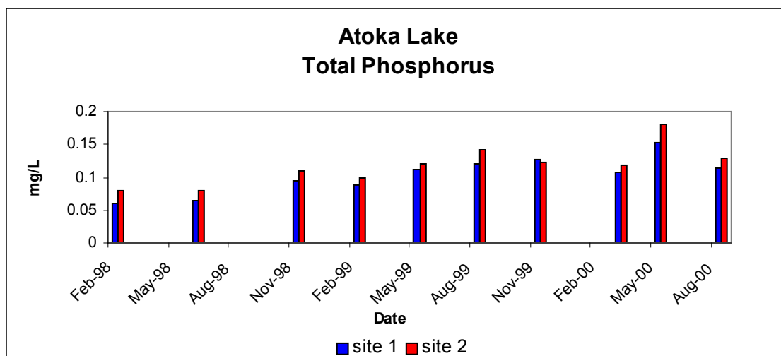
Figure 56. Atoka Lake TP concentration, November 1997 through August 2000.
