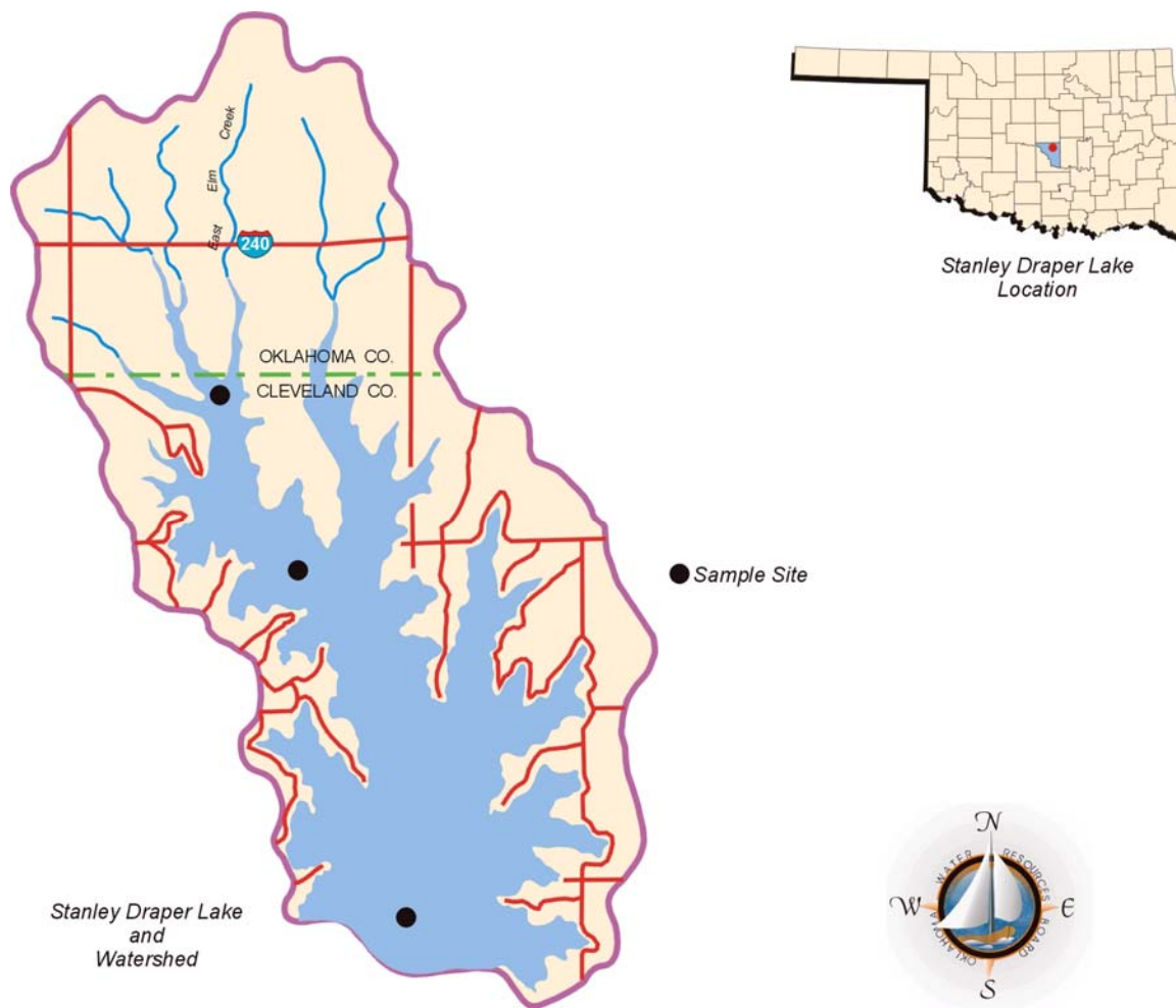
Figure 5. Location of Lake Stanley Draper and its watershed.
