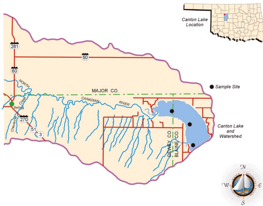
Figure 2. Location of Canton Lake and its watershed.
