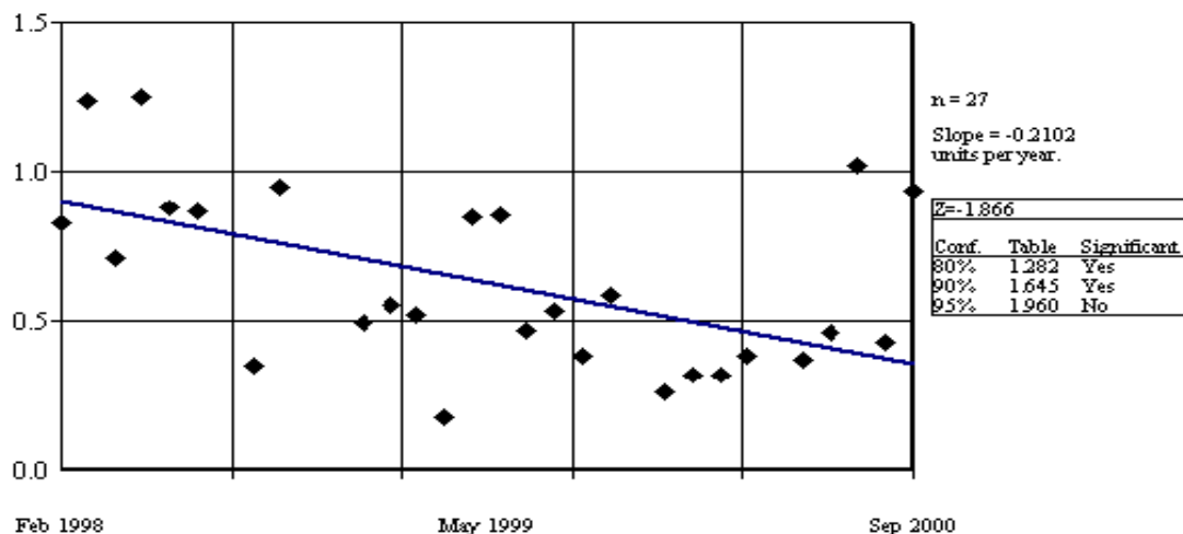
Figure 11. Trend analysis for flow-adjusted total nitrogen data collected from February of 1998 through September of 2000 at the Beaver River near Beaver, OK. Slope calculated using the Seasonal Kendall slope estimator. Data deseasonalized based on three seasons beginning February 1, June 1, and October 1. Values on Y-axis are LOWESS calculated residuals.
