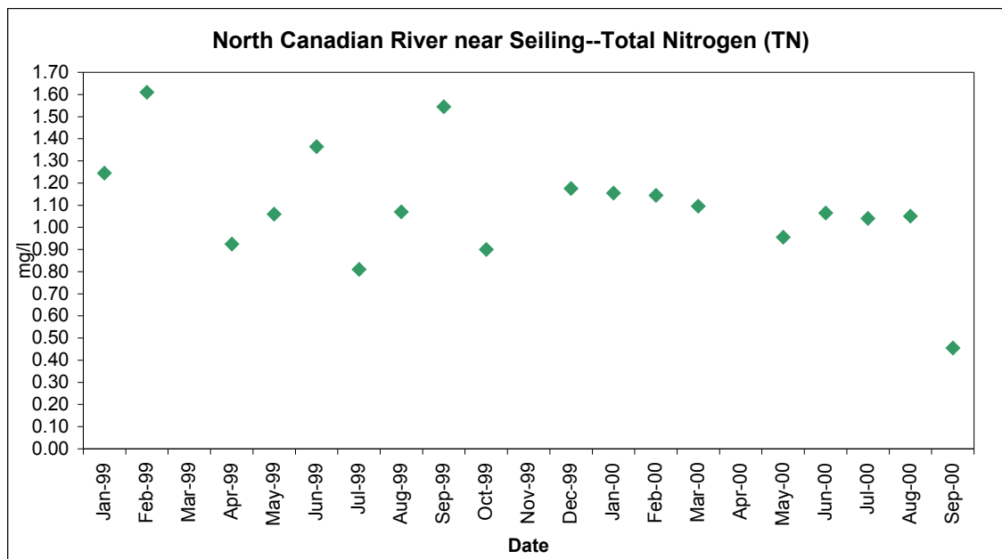
Figure 13. Total nitrogen and total phosphorus data collected at North Canadian River near Seiling, OK, from January 1999 through September of 2000.
