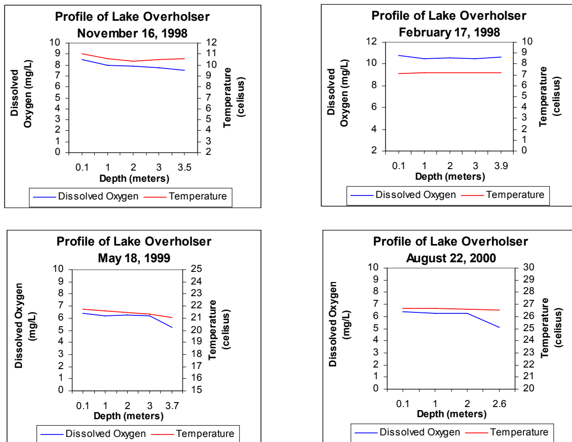
Figure 34. Vertical dissolved oxygen and temperature profiles representing four seasons measured at Site 1 in Lake Overholser.
