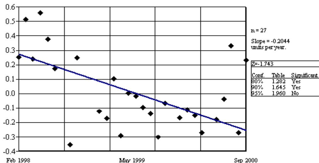
Figure 11. Trend analysis for flow-adjusted total nitrogen data collected from February of 1998 through September of 2000 at the Beaver River near Beaver, OK. Slope calculated using the Seasonal Kendall slope estimator. Data deseasonalized based on three seasons beginning February 1, June 1, and October 1. Values on Y-axis are LOWESS calculated residuals.
