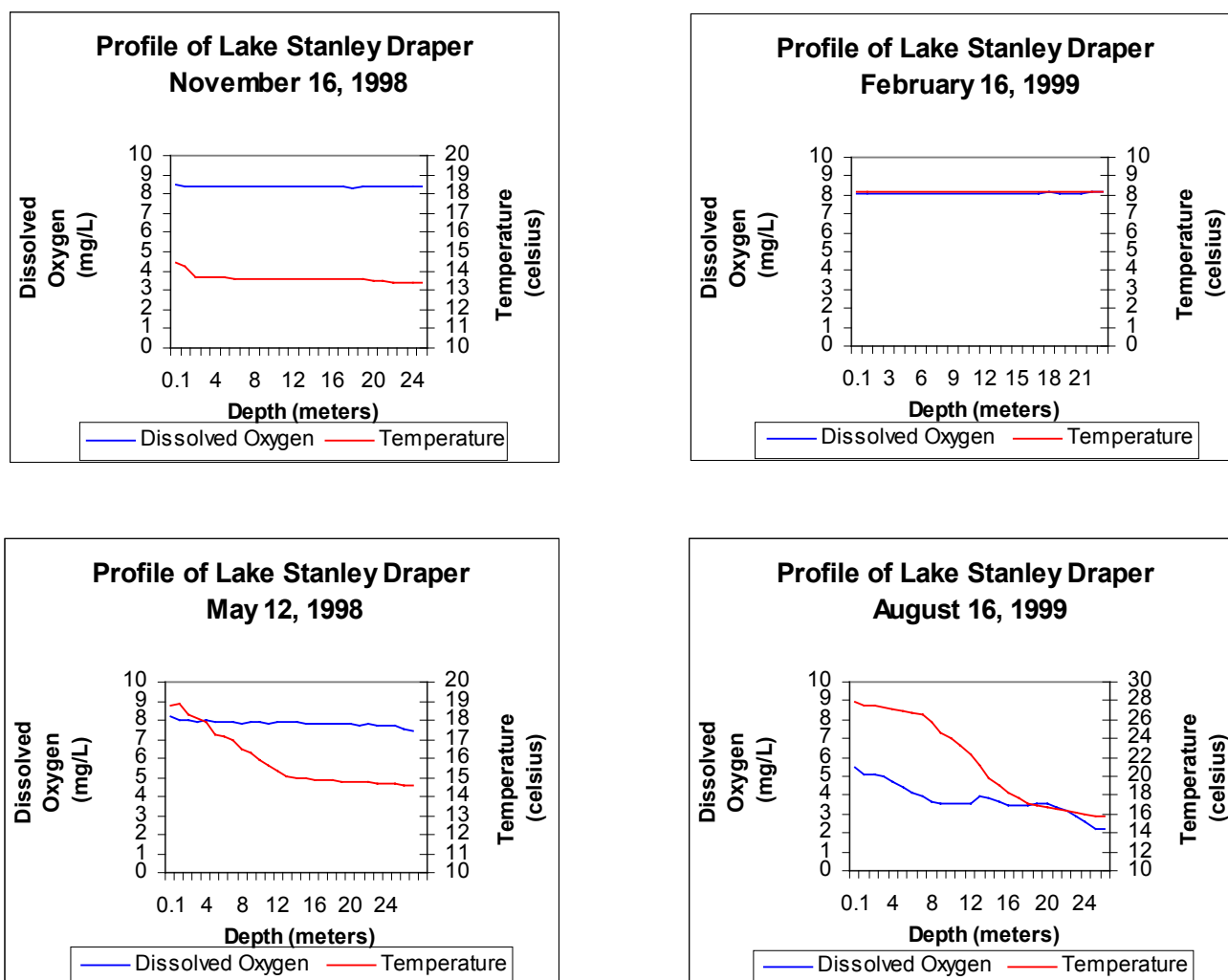
Figure 48. Vertical dissolved oxygen and temperature profiles representing four seasons measured at Site 1 in Lake Stanley Draper.
