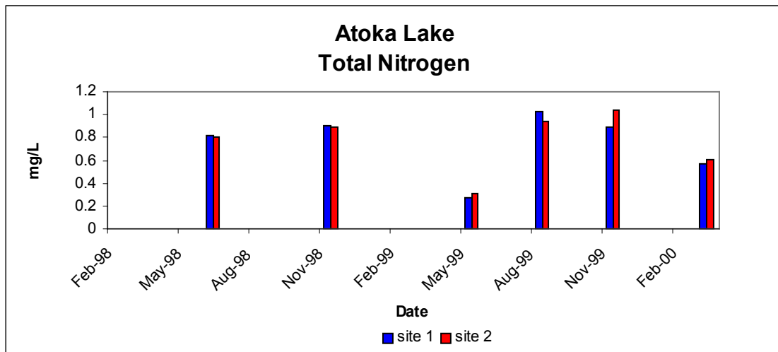
Figure 56. Atoka Lake TN concentration, November 1997 through August 2000.
