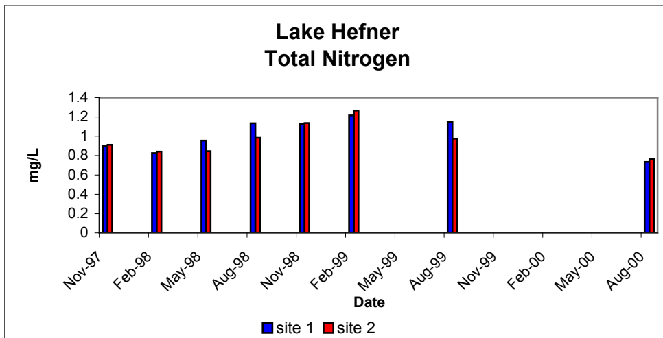
Figure 42. Lake Hefner TN concentrations, November 1997 through August 2000.
