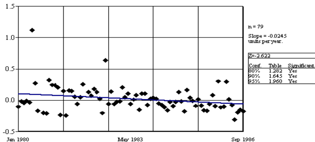
Figure 16. Trend analysis for flow-adjusted historical total phosphorus data collected from January of 1980 through September of 1986 at the North Canadian River near Seiling, OK. Slope calculated using the Seasonal Kendall slope estimator. Data deseasonalized based on three seasons beginning February 1, July 1, and October 1. Values on Y-axis are LOWESS calculated residuals.
