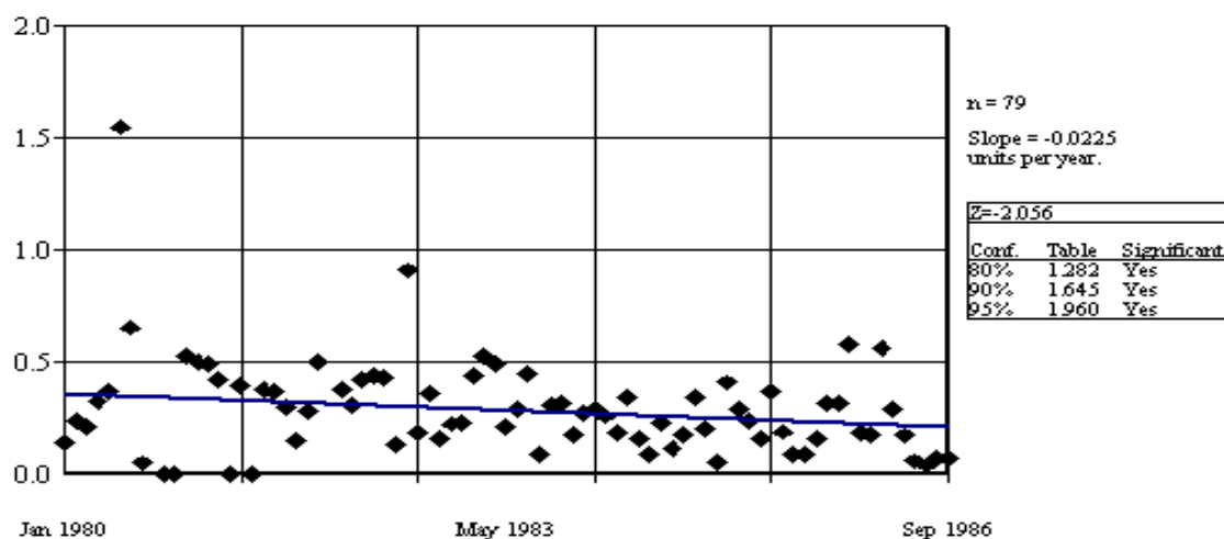
Figure 15. Trend analysis for raw historical total phosphorus data collected from January of 1980 through September of 1986 at the North Canadian River near Seiling, OK. Slope calculated using the Seasonal Kendall slope estimator. Data deseasonalized based on three seasons beginning February 1, July 1, and October 1. Values on Y-axis are LOWESS calculated residuals.
