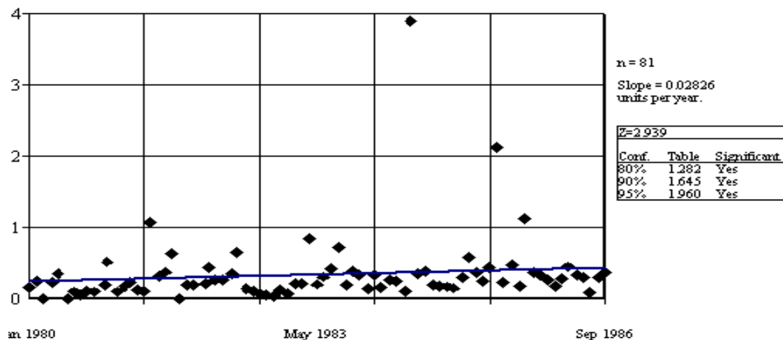
Figure 19. Trend analysis for raw historical total phosphorus data collected from January of 1980 through September of 1986 at the North Canadian River near El Reno, OK. Slope calculated using the Seasonal Kendall slope estimator. Data deseasonalized based on three seasons beginning February 1, July 1, and October 1. Values on Y-axis are LOWESS calculated residuals.
