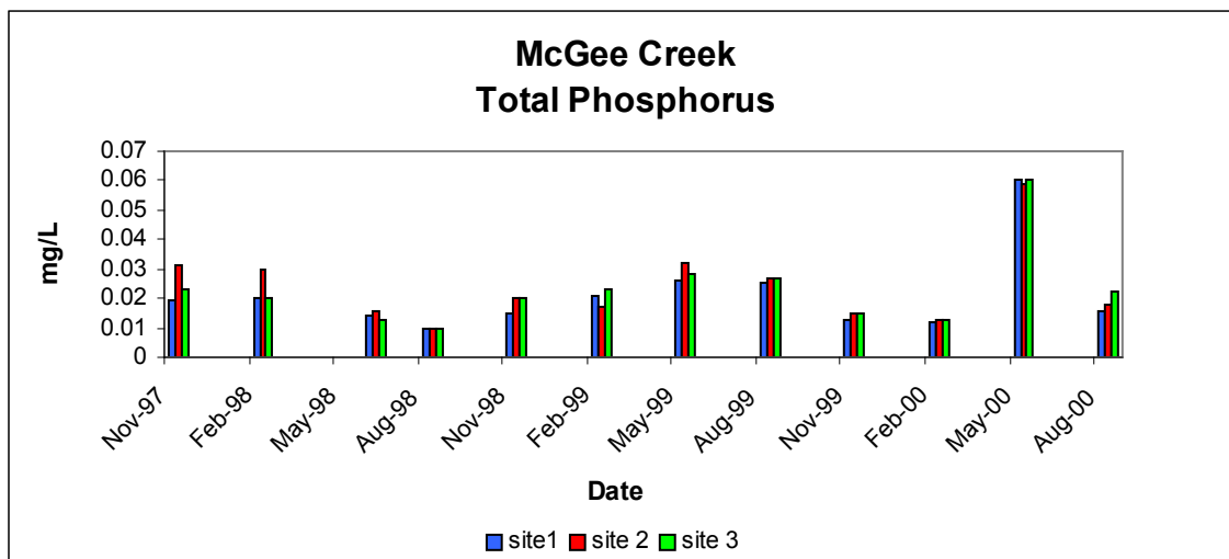
Figure 64. McGee Creek TP concentrations, November 1997 through August 2000.
