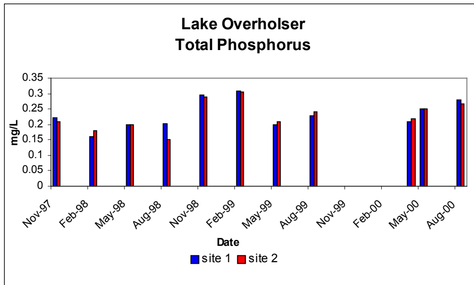
Figure 36. Lake Overholser TP concentrations, November 1997 through August 2000.
