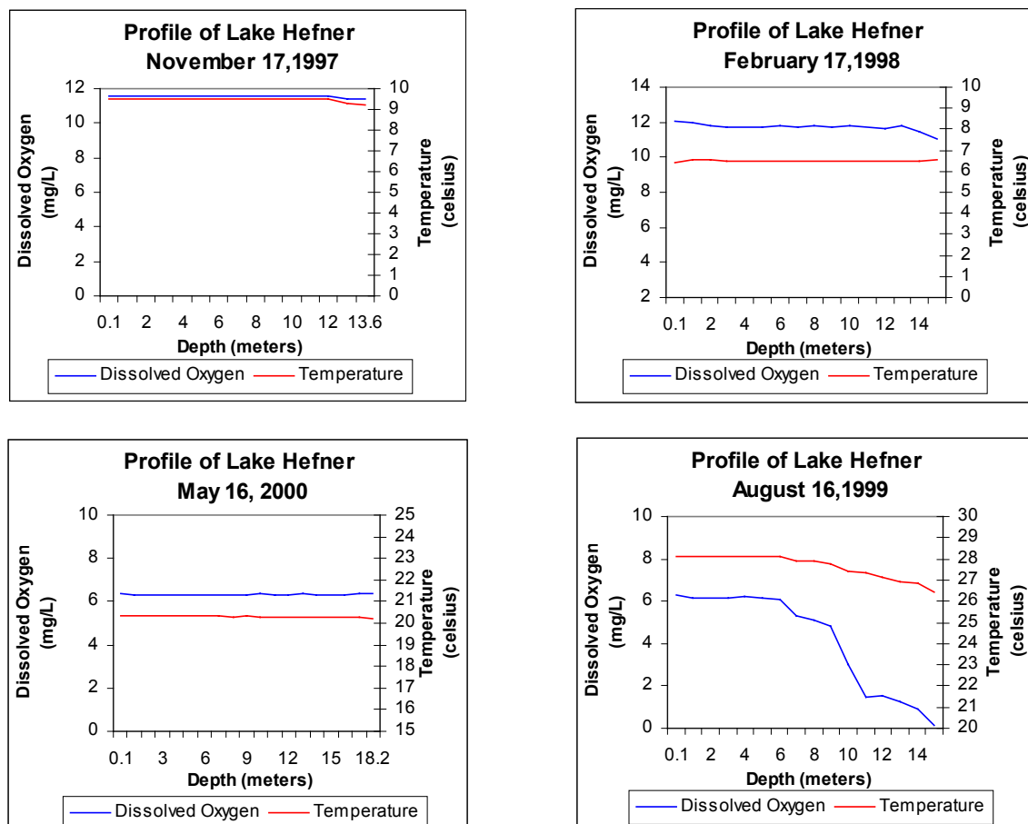
Figure 41. Vertical dissolved oxygen and temperature profiles measured at the lacustrine site at Lake Hefner representing four seasons sampled.
