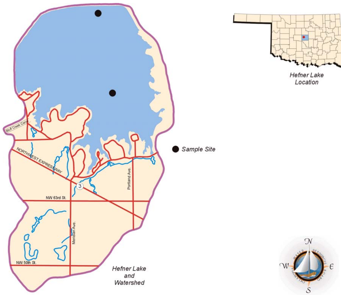
Figure 4. Location of Hefner Lake and its watershed.
