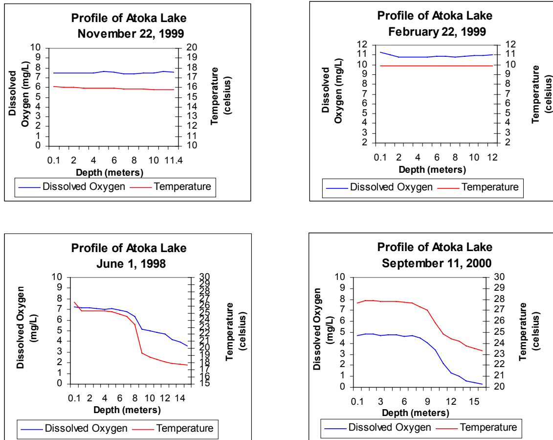
Figure 55. Vertical dissolved oxygen and temperature profiles representing four seasons measured at Site 1 in Atoka Lake
