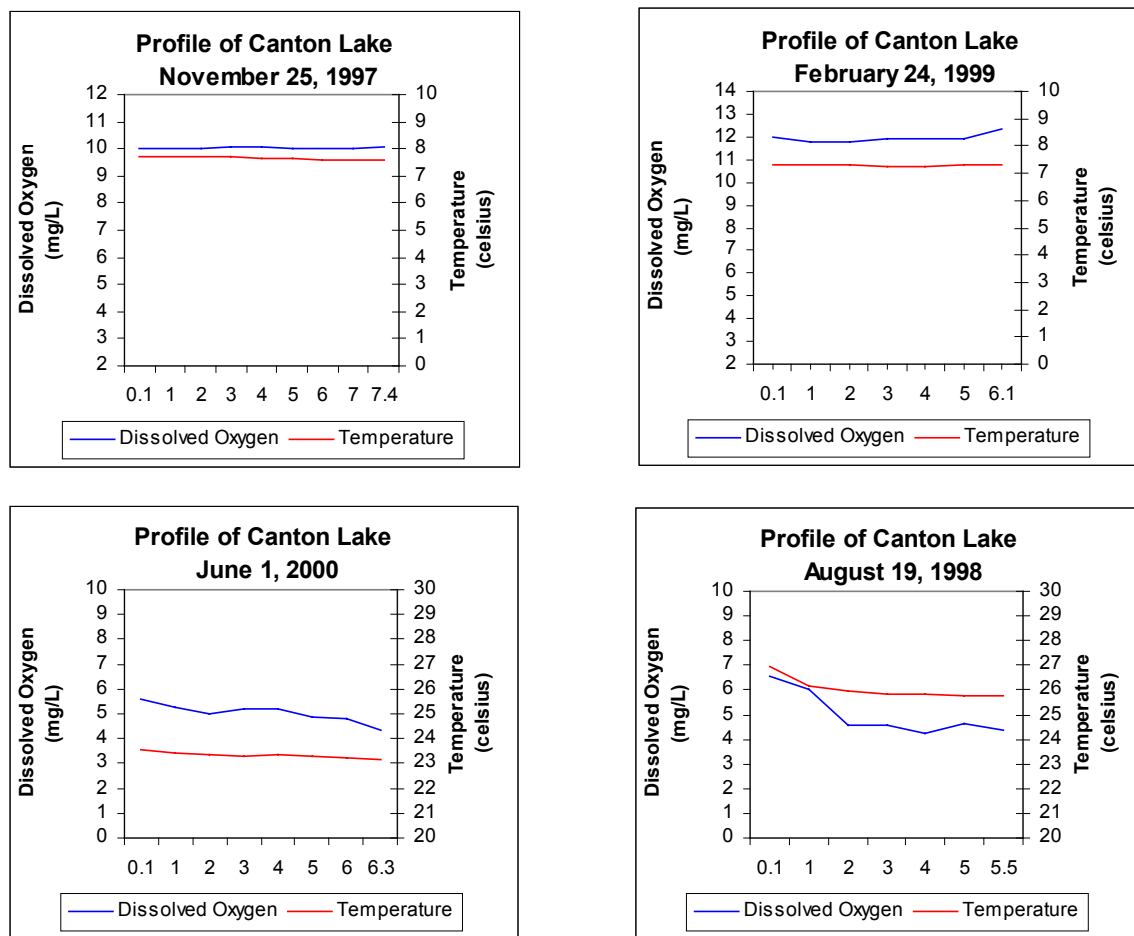
Figure 27. Vertical dissolved oxygen and temperature profiles representing four seasons measured at Site 1 in Canton Lake.
