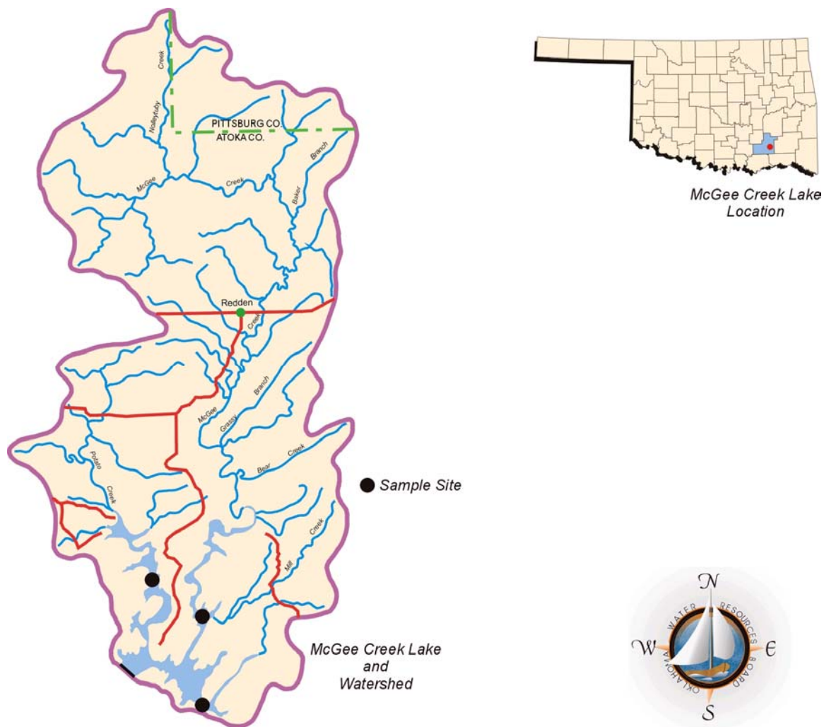
Figure 7. Location of McGee Creek Reservoir and its watershed.
