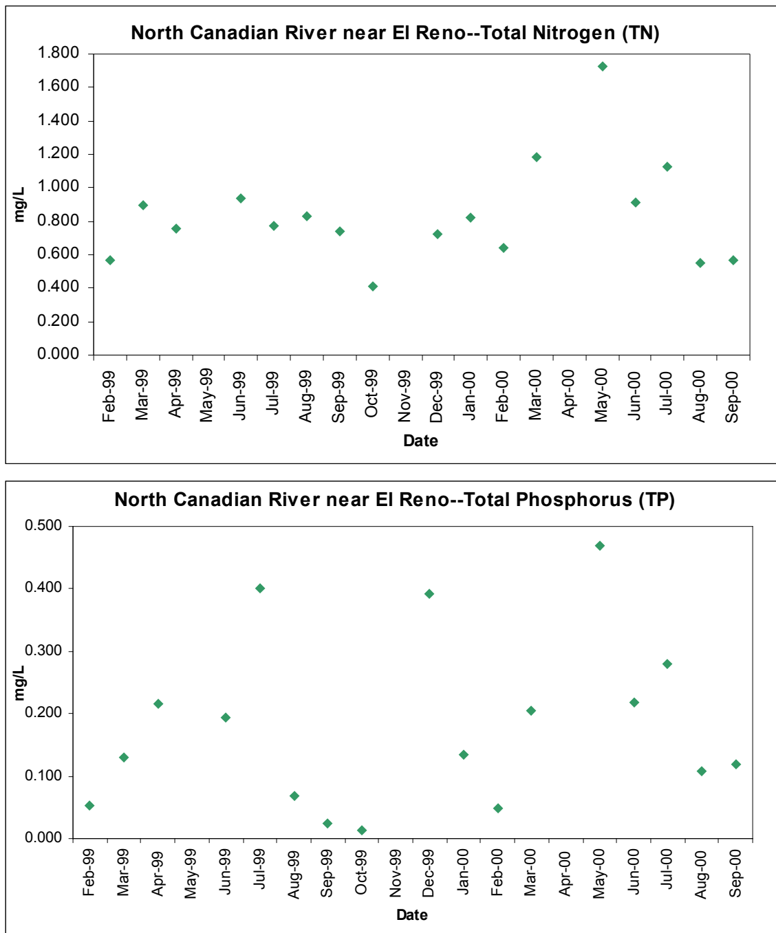
Figure 18. Total nitrogen and total phosphorus data collected at North Canadian River near El Reno, OK, from February 1999 through September of 2000.
