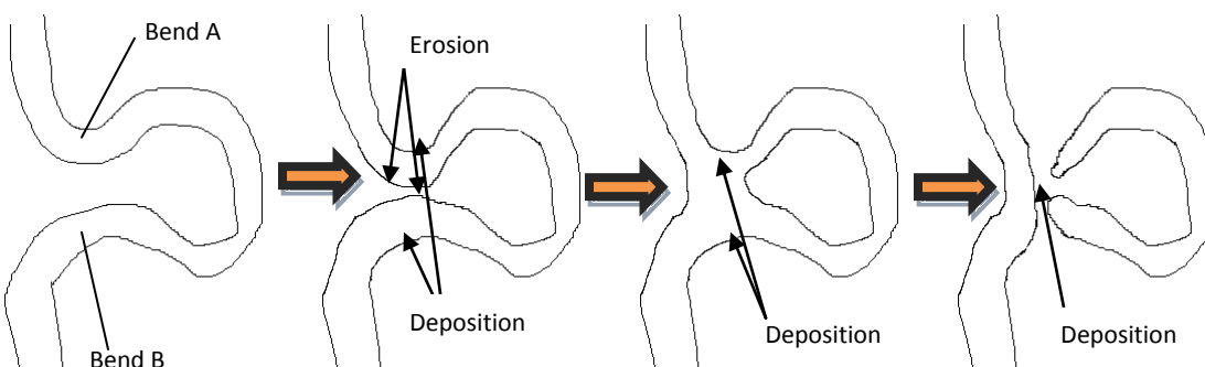
Figure 1: Oxbow formation showing erosional and depositional processes in a meander over time.
