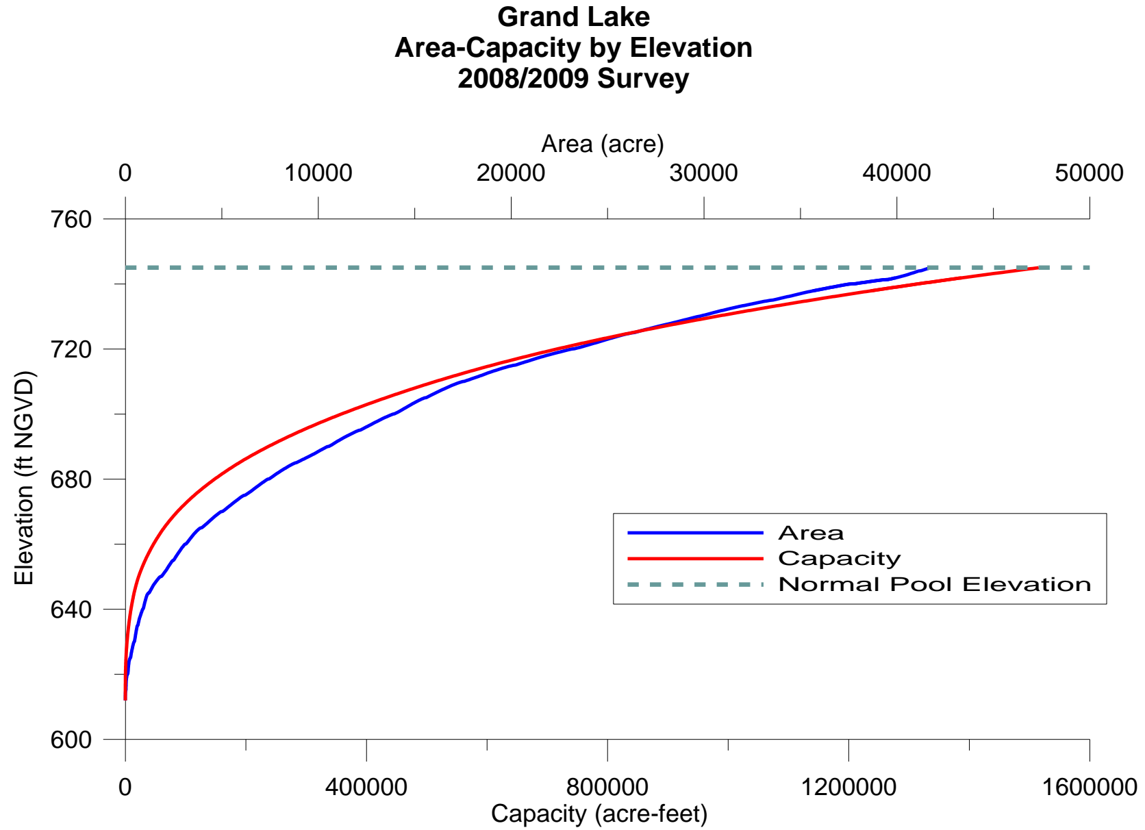
Figure A. 1. Area-Capacity Curve for Grand Lake
